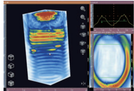
TFM 3D real-time imaging for bolt
