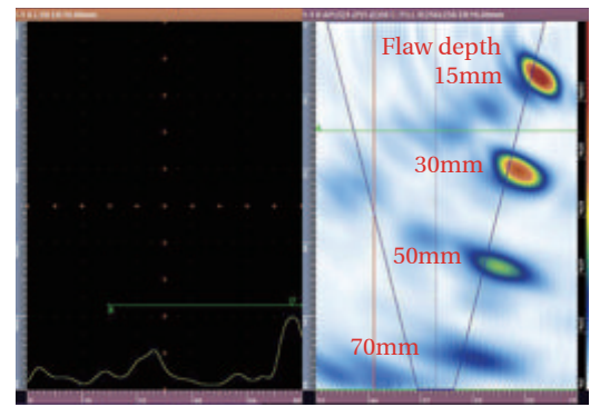
Austenitic block with DMA probe (Thickness 80mm)
