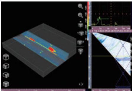
PA 3D: Supports 3D display of workpiece, probe, wedge, beam simulation and flaws.
