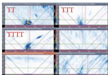
Incomplete root penetration
