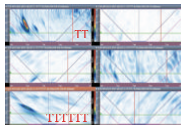
Lack of fusion
