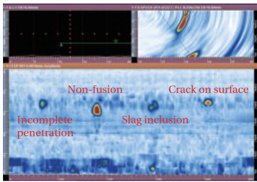
Austenitic plate with DLA probe (Thickness 40mm)
