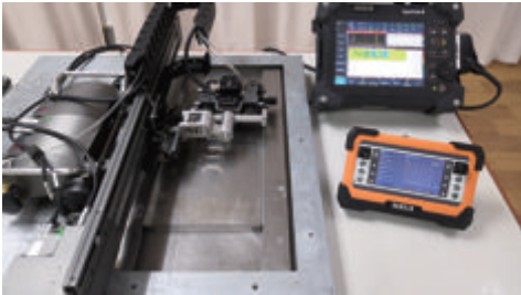
Automated 2-axis scanning
