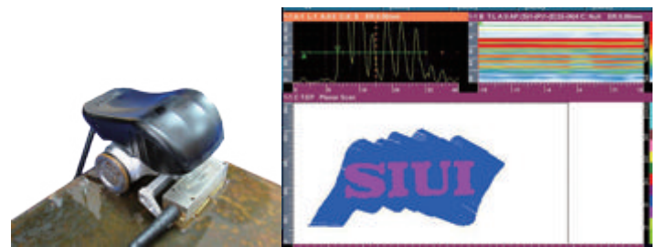
Free 2D scanning
