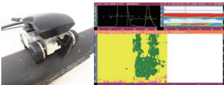
PA immersion testing
