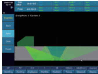
Beam Coverage Simulation
