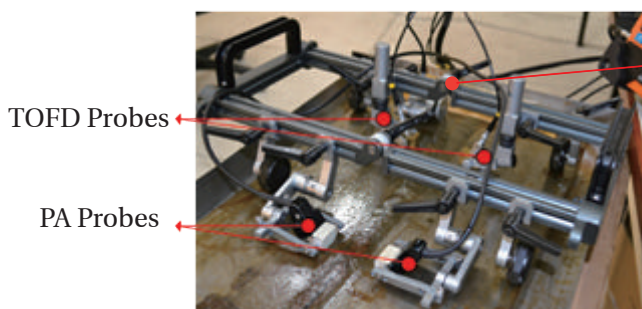
Foldable Mechanism
