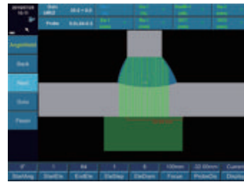
T-weld Simulation
