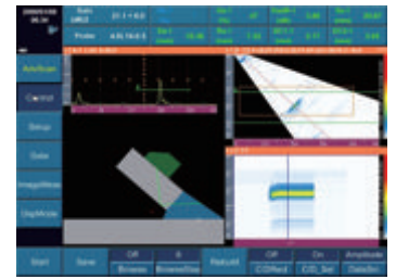
RayTracing (A+B+C+R Scan)
