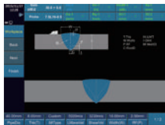
Workpiece Setup
