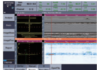
TOFD+Conventional UT to inspect the blind zone area
