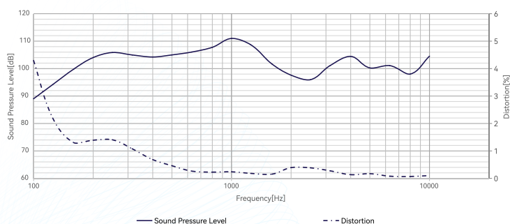
Fig.1 CRY3602 Mouth Simulator Set Typical Frequency Response and Distortion at 1V
