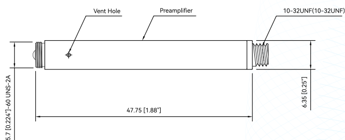
Fig.1 CRY3543 preamplifier Drawings
