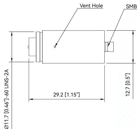
Fig.1 CRY3502 preamplifier Drawings
