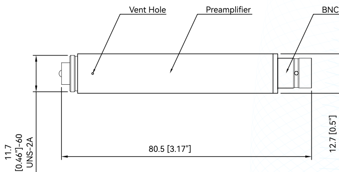
Fig.1 CRY3501 preamplifier Drawings
