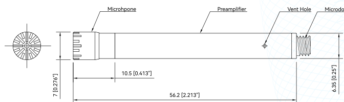
Fig.2 CRY3404-S01 Microphone Set Drawings
