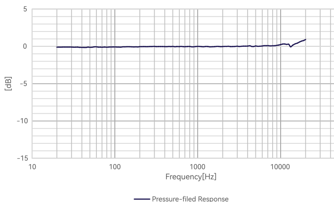
Fig.1 CRY3404-S01 Microphone Set Typical Frequency Response
