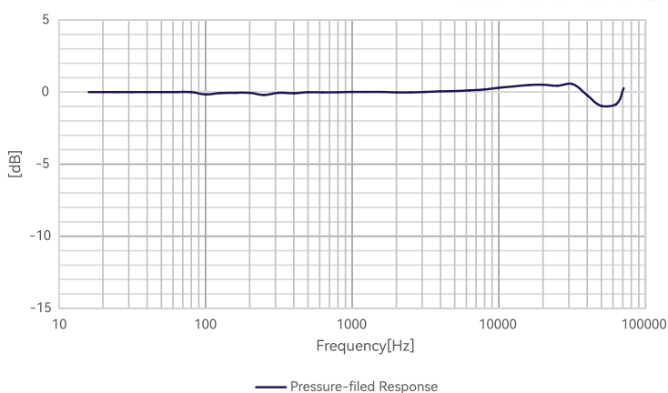
Fig.2 CRY3402 Microphone Typical Frequency Response
