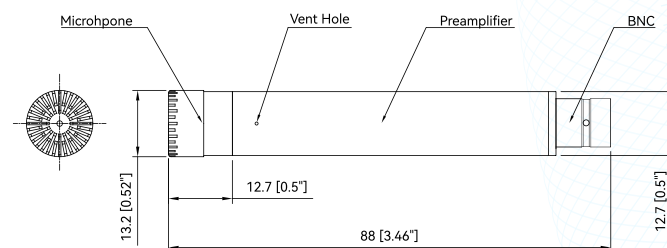
Fig.2 CRY3202-S01 Microphone Set Drawings
