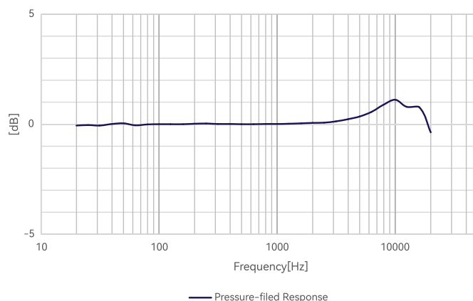
Fig.1 CRY3202-S01 Microphone Set Typical Frequency Response
