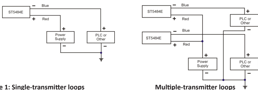
Figure 1: Single-transmitter loops
