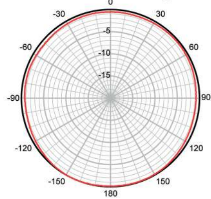
Horizontal Beam Pattern @ 60kHz
