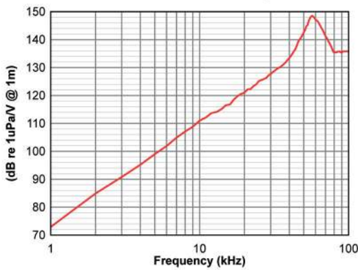
Transmit Sensitivity
