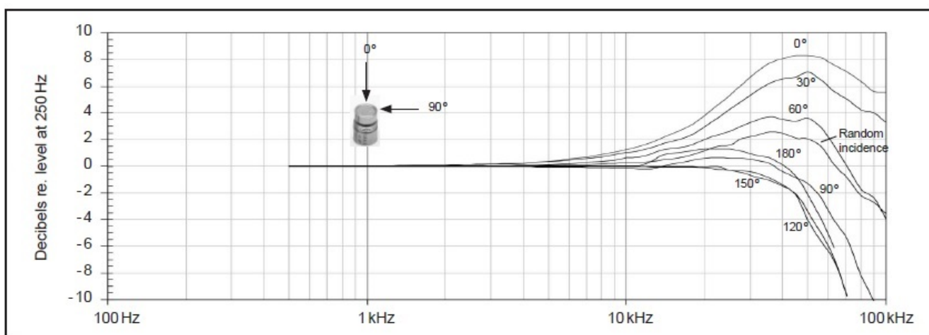
Free-field corrections for different angles of incidence
