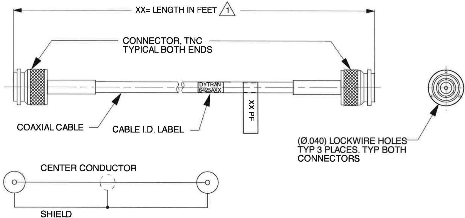
SCHEMATIC DIAGRAM
