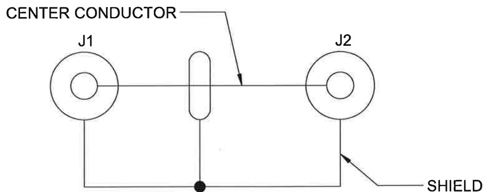
SCHEMATIC DIAGRAM
