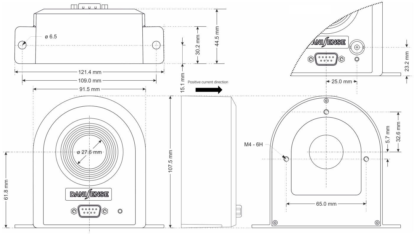
Figure 5: Dimensions of sensor head. Tolerance is 0.3 mm
